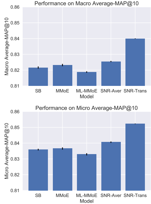
Figure 2: Accuracy of Best-Tuned Models. The bar chart shows the average test performance of the top 10 models selected on validation set. The error bar indicates the standard error of the average test performance.
